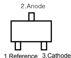
SOT-23 (Front View)
